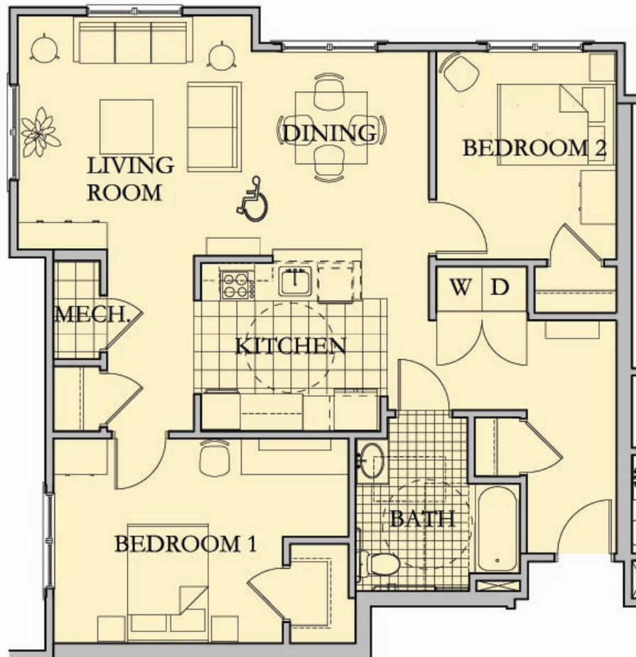
TYPICAL UNIT PLAN TYPE 2E (BF) 2 BDRM., 1 BATH N.T.S. APPROXIMATELY 1,032 SF
