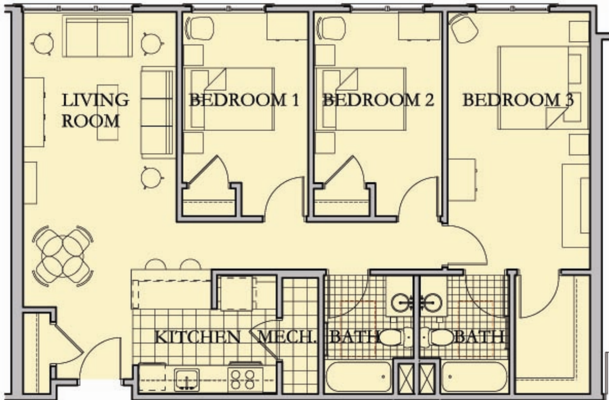
TYPICAL UNIT PLAN TYPE 3A 3 BDRM., 2 BATH N.T.S. APPROXIMATELY 1,123 SF
